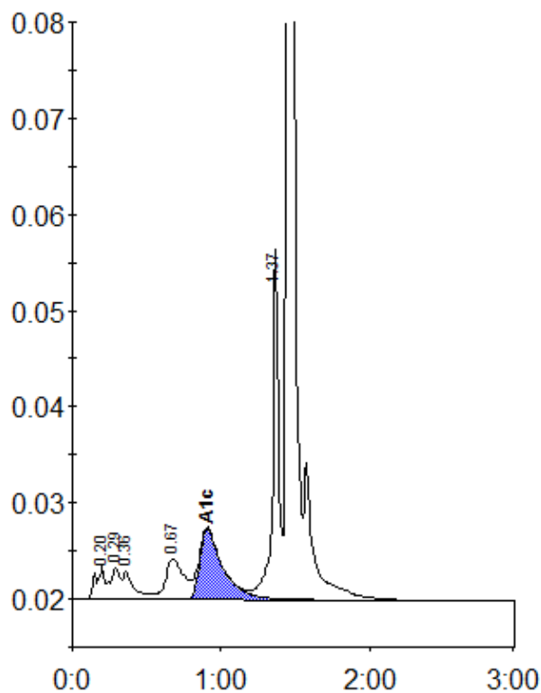
Peak table - ID: 10468508
